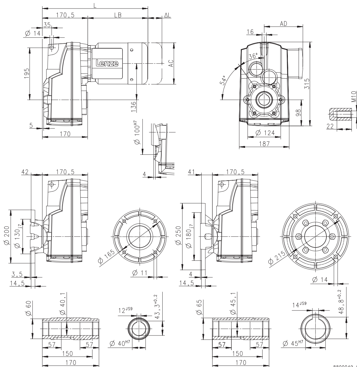
Dimensions with hollow shaft
